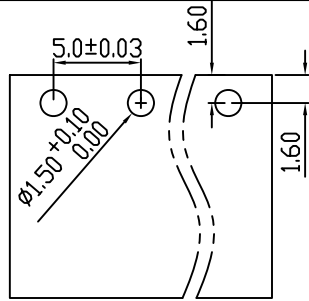
PCB LAYOUT
