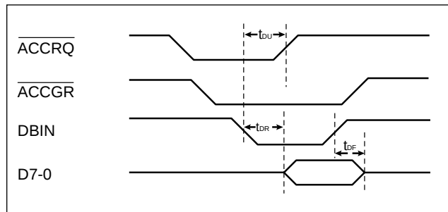
Figure 6. DMA Read
