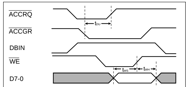
Figure 8. DMA Write
