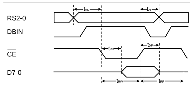
Figure 5. CPU Read
