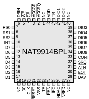
Pin Configuration
