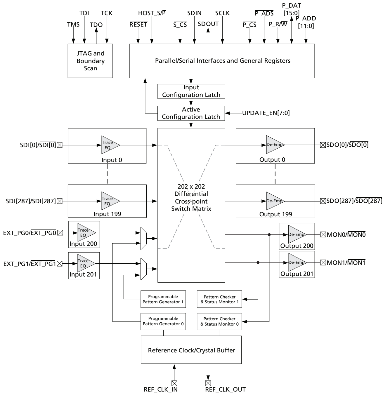
GX3202 Functional Block Diagram
