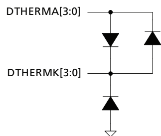
Figure 4-3: Temperature Sensors
