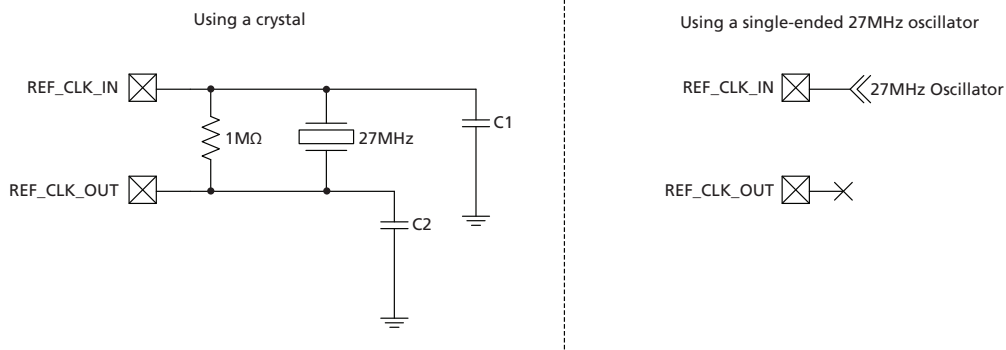
Figure 3-5: Crystal Oscillator
