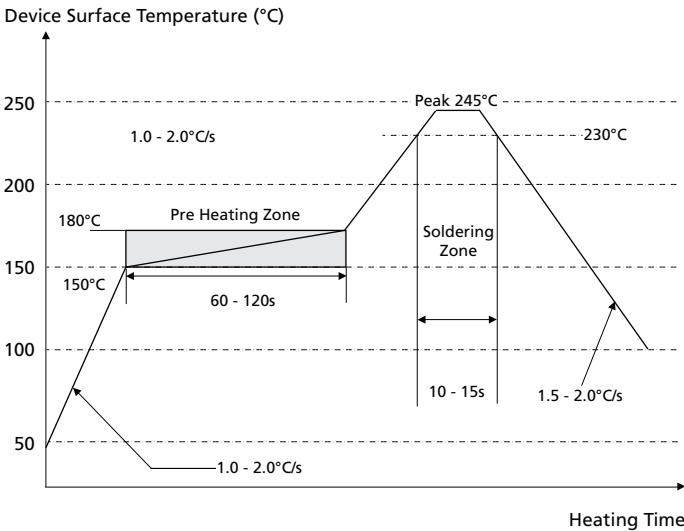
Figure 6-1: Maximum Pb-free Solder Reflow Profile
