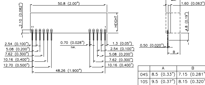
BACK VIEW
