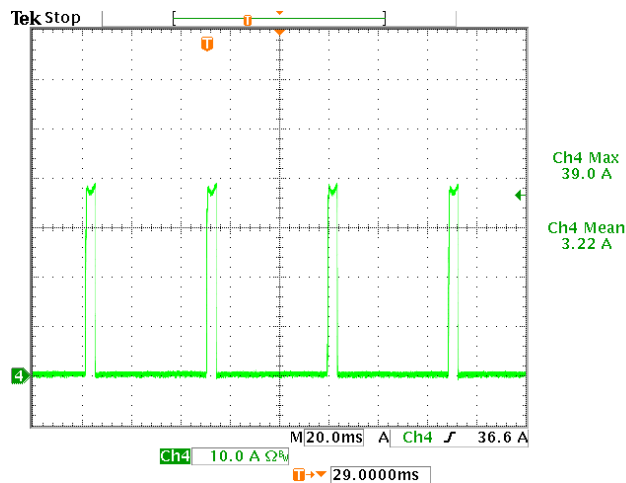
Figure 27: Output short circuit current 5\text{V}_{in}, 0.75\text{V}_{out}
