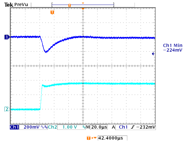
Figure 26: Typical Transient Response to Step Load Change at 2.5\text{A}/\mu\text{S} from 50% to 100% of I_o , max at 3.3\text{V}_{in}, 1.8\text{V}_{out} ( C_{out} = 1\mu\text{F} ceramic, 10\mu\text{F} Tantalum)
