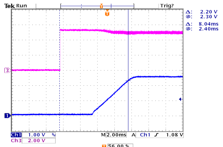
Figure 18: Turn on delay time at remote turn on with external capacitors (Co= 5000 μF) 3.3Vin, 2.5V/16A out
