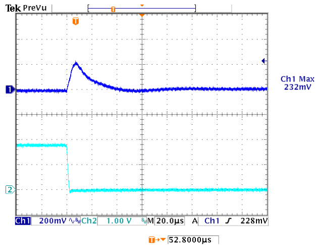
Figure 25: Typical Transient Response to Step Load Change at 2.5\text{A}/\mu\text{S} from 100% to 50% of I_o , max at 3.3\text{V}_{in}, 1.8\text{V}_{out} ( C_{out}=1\mu\text{F} ceramic, 10\mu\text{F} Tantalum)
