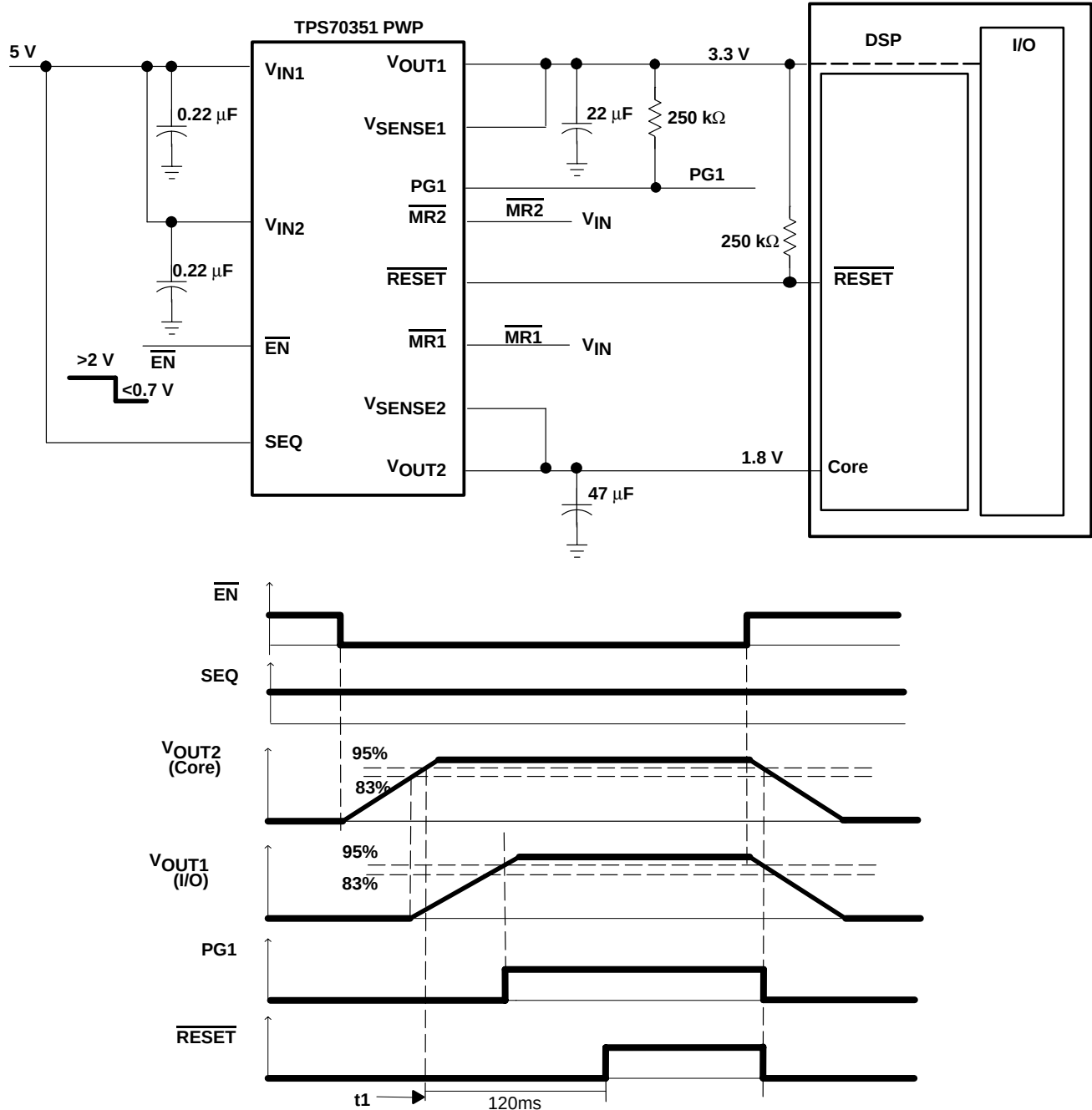
Figure 44. Application Timing Diagram (SEQ = High)
