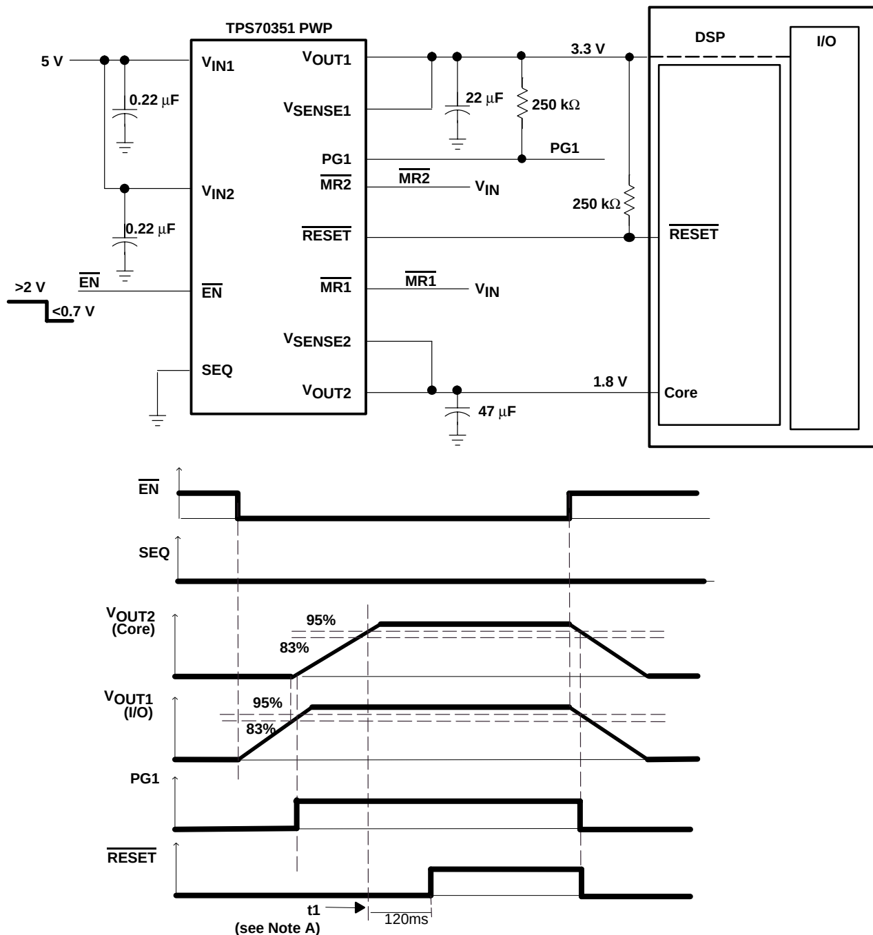
Figure 43. Application Timing Diagram (SEQ = Low)
