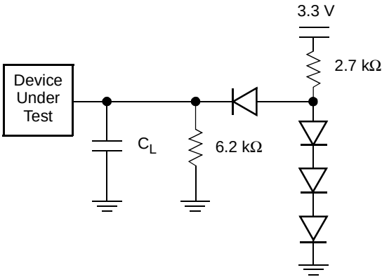
Figure 11. Test Setup
