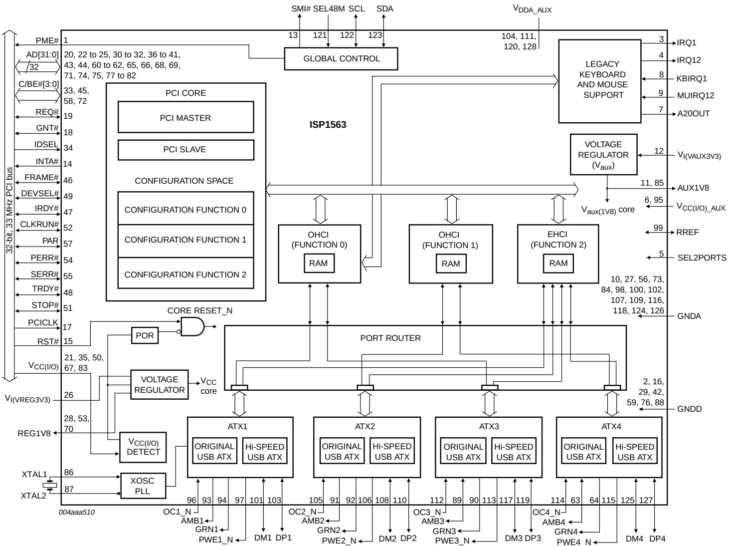
Fig 1. Block diagram.
