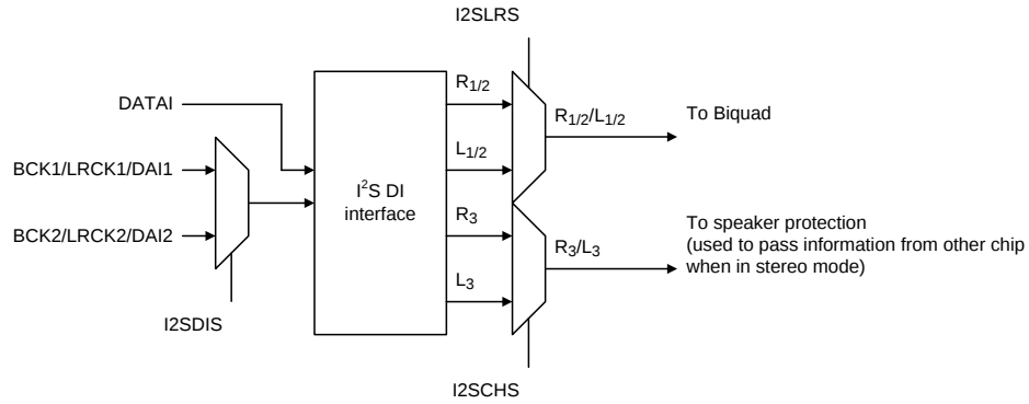
Figure 11. I²S Input Mux
