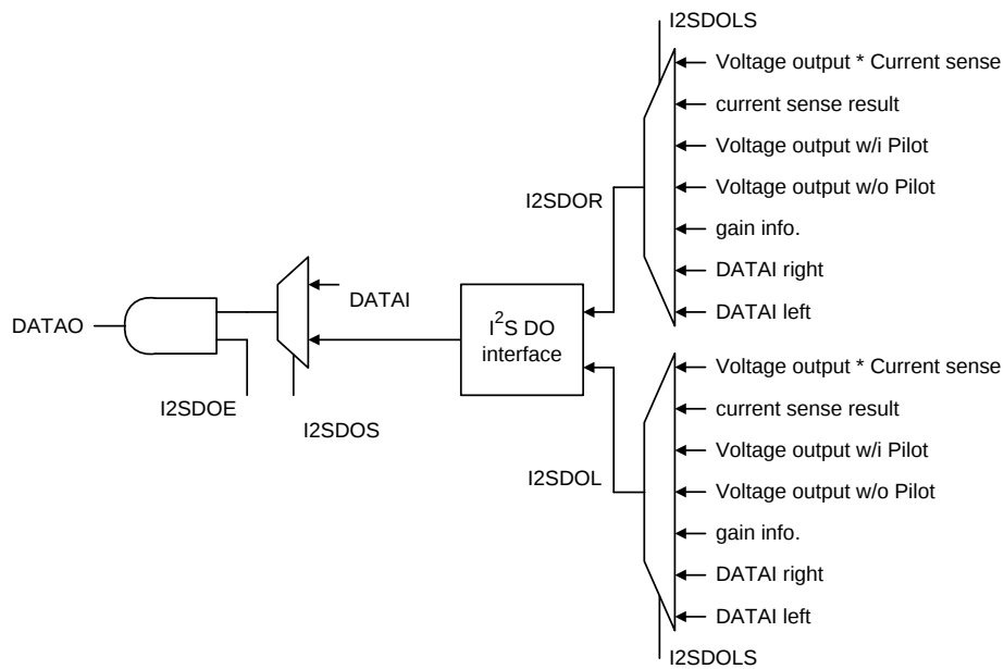
Figure 12. I²S Output Mux
