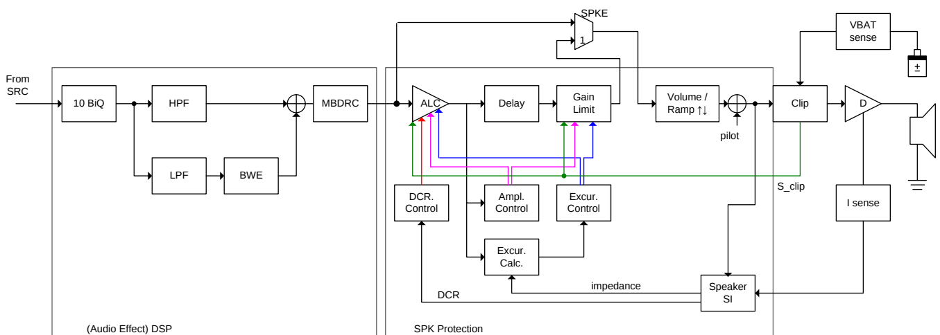
Figure 13. Signal Processing Path
