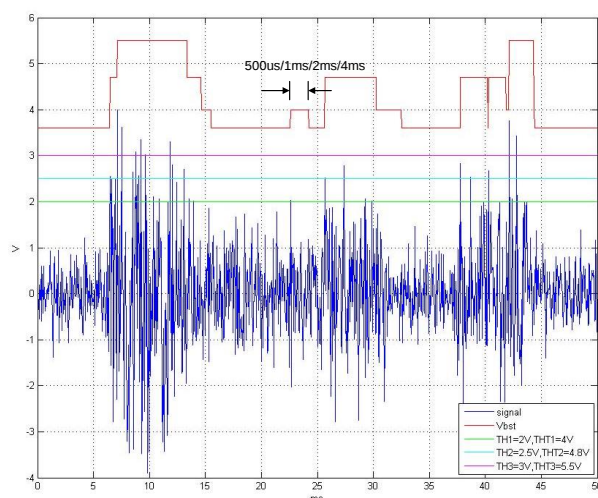
Figure 23. Illustration for Adaptive Boost Mode
