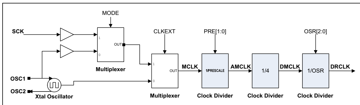
FIGURE 4-1: Clock Sub-Circuitry.
