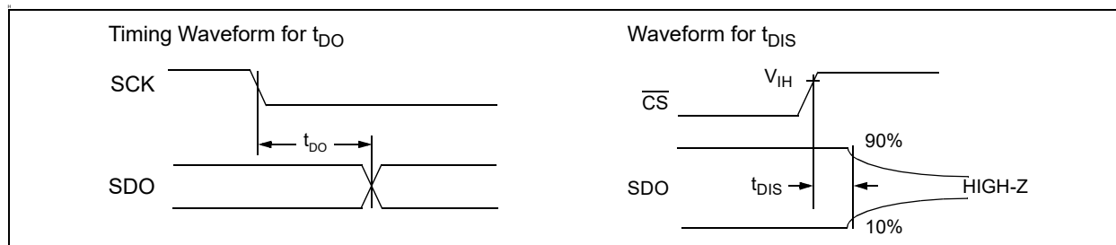
FIGURE 1-4: Timing Waveforms.
