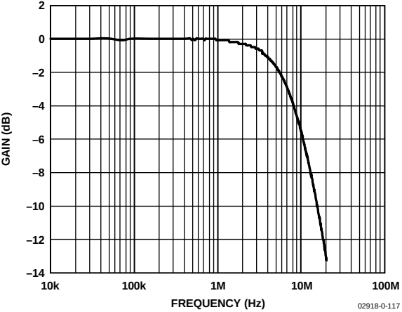
Figure 14. Reference Multiplying Bandwidth
