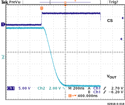
Figure 15. Settling Time
