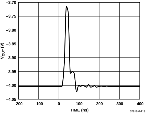
Figure 16. Midscale Transition and Digital Feedthrough
