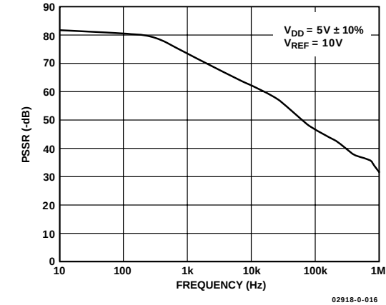
Figure 12. Power Supply Rejection Ration vs. Frequency
