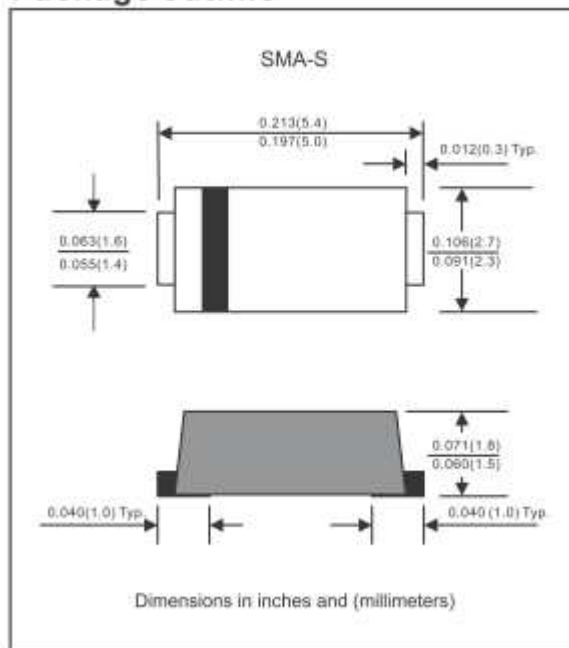
Package outline
