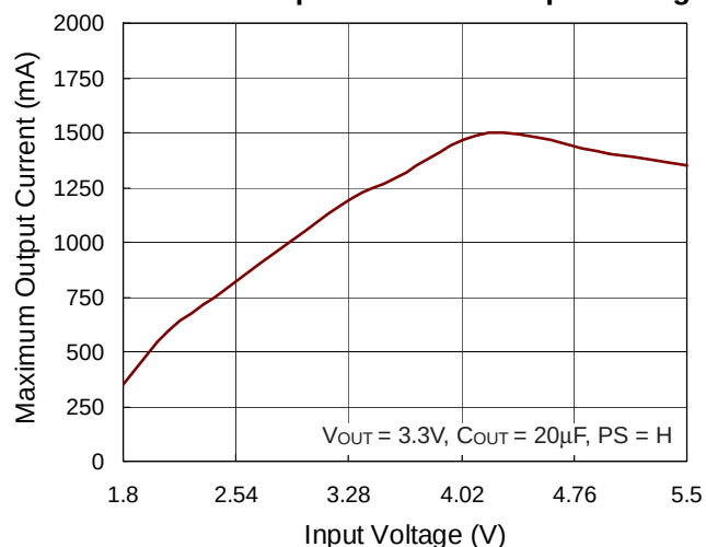
Maximum Output Current vs. Input Voltage
