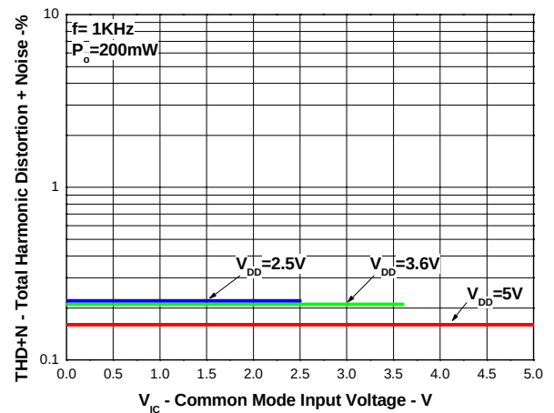
TOTAL HARMONIC DISTORTION+NOISE vs COMMON MODE INPUT VOLTAGE
