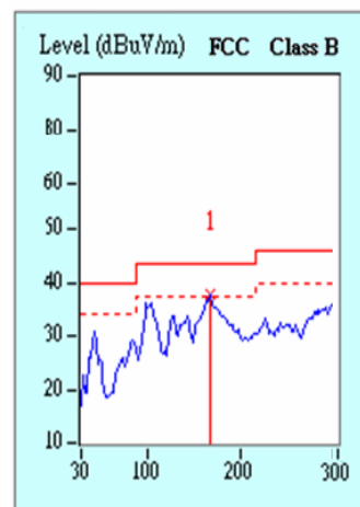
Figure29. EMI Test and FCC Limits
