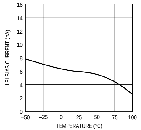
LB1 Bias Current vs Temperature
