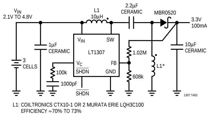
Step-Up/Step-Down Converter
