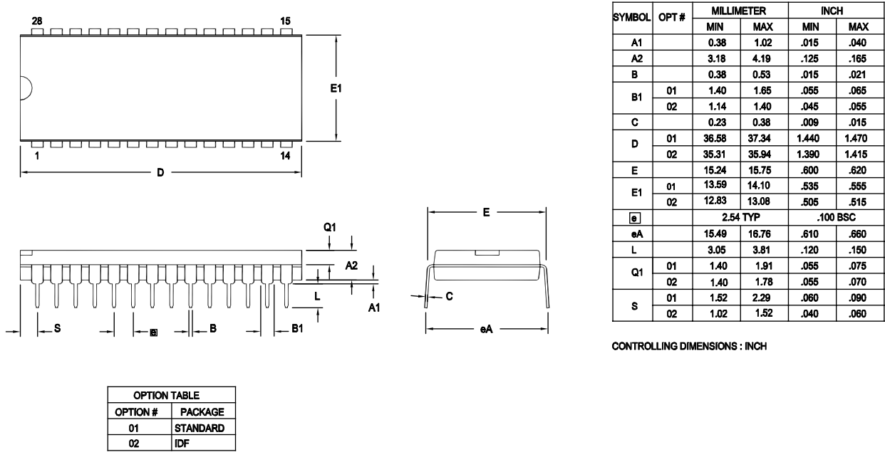
Figure 45 illustrates the 28-pin Plastic Dual Inline Package (PDIP) available for the Z8 Encore! XP® 4K Series devices.
