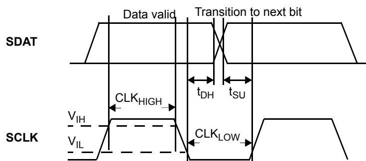
Figure 2. Data Valid and Data Transition Periods
