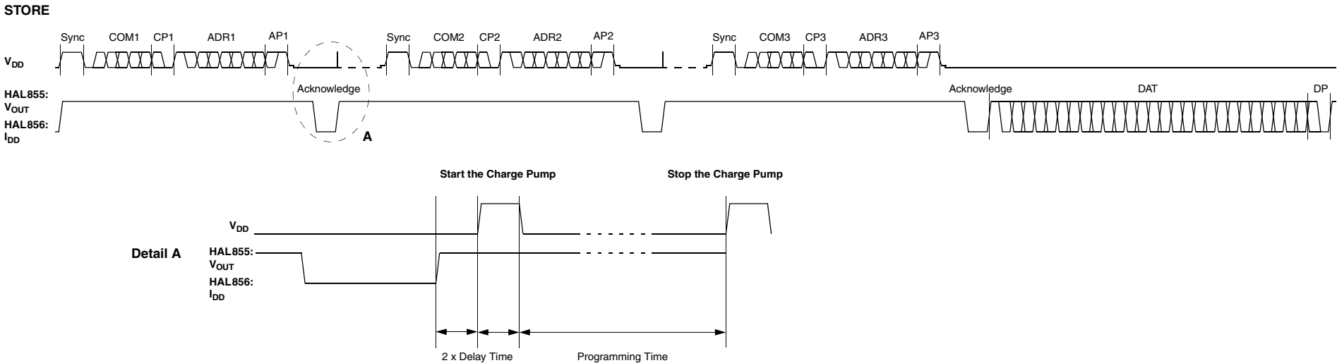
Fig. 6–5: Telegram for programming the EEPROM
