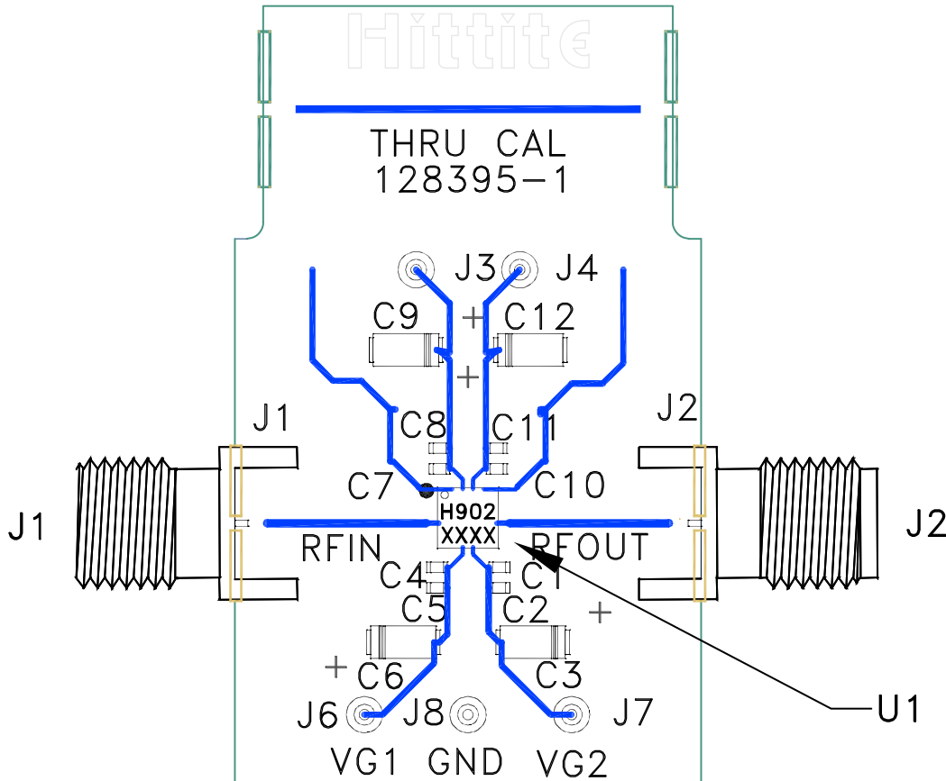
Figure 22. Evaluation PCB (128395-1)
