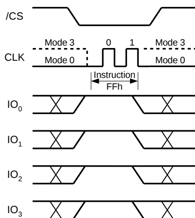
Figure 51. Exit QPI Instruction (QPI Mode only)
