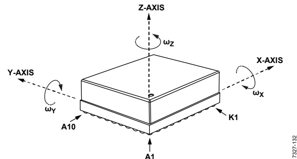
Figure 41. Gyroscope Axis and Polarity Assignments
