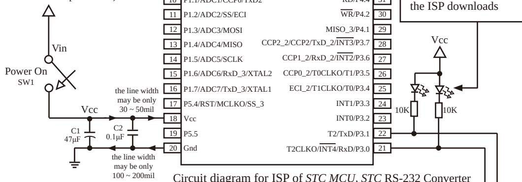
Circuit diagram for ISP of STC MCU , STC RS-232 Converter
