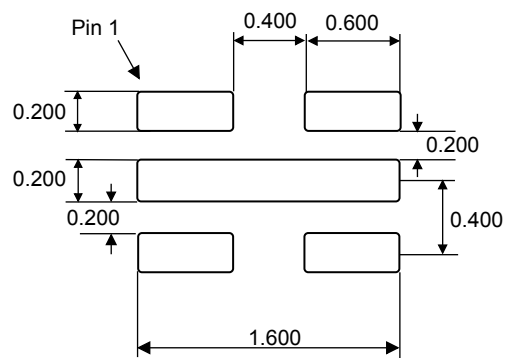
Figure 31. UFDFPN5 - Recommended footprint
