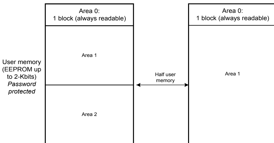
Figure 5. Memory organization
