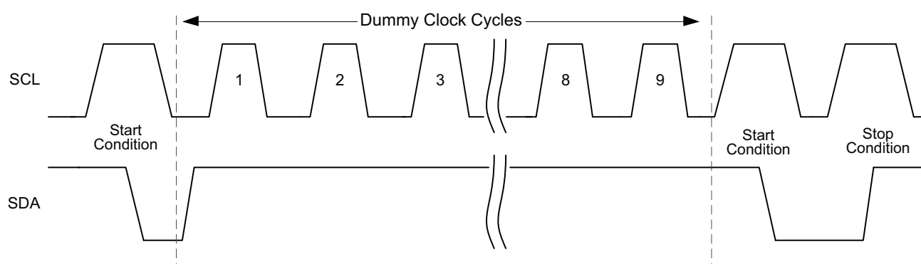
Figure 7-4. Software Reset
