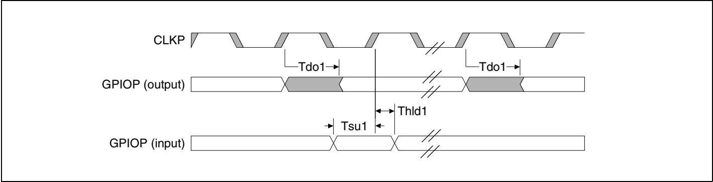
Figure 16 GPIO AC Timing Waveform
