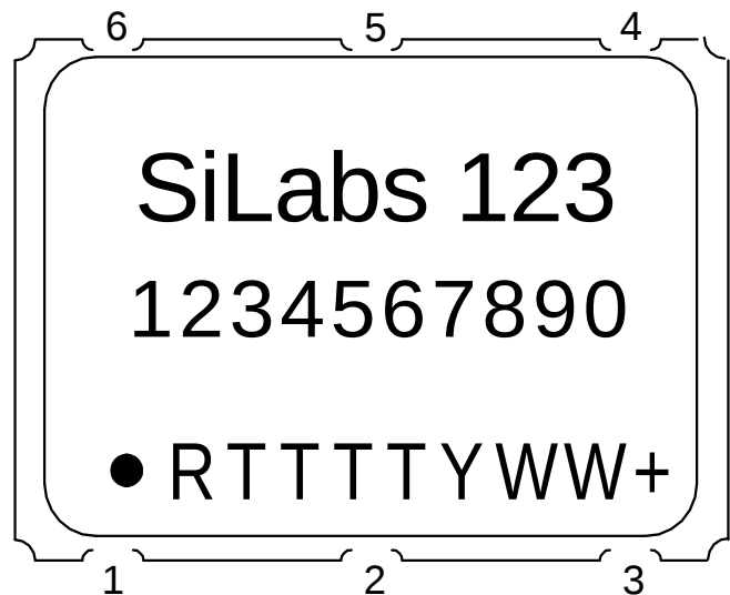
Figure 3. Mark Specification
