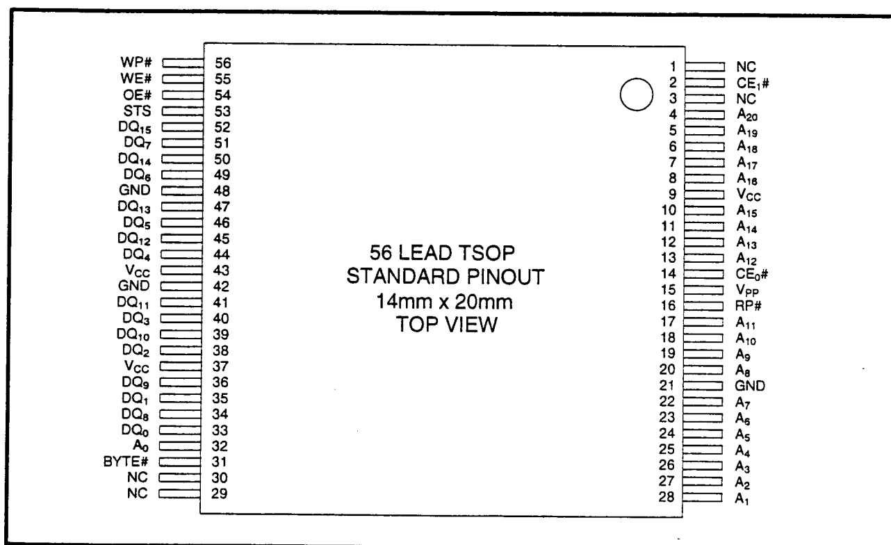
Figure 3. TSOP 56-Lead Pinout (Reverse Bend)
