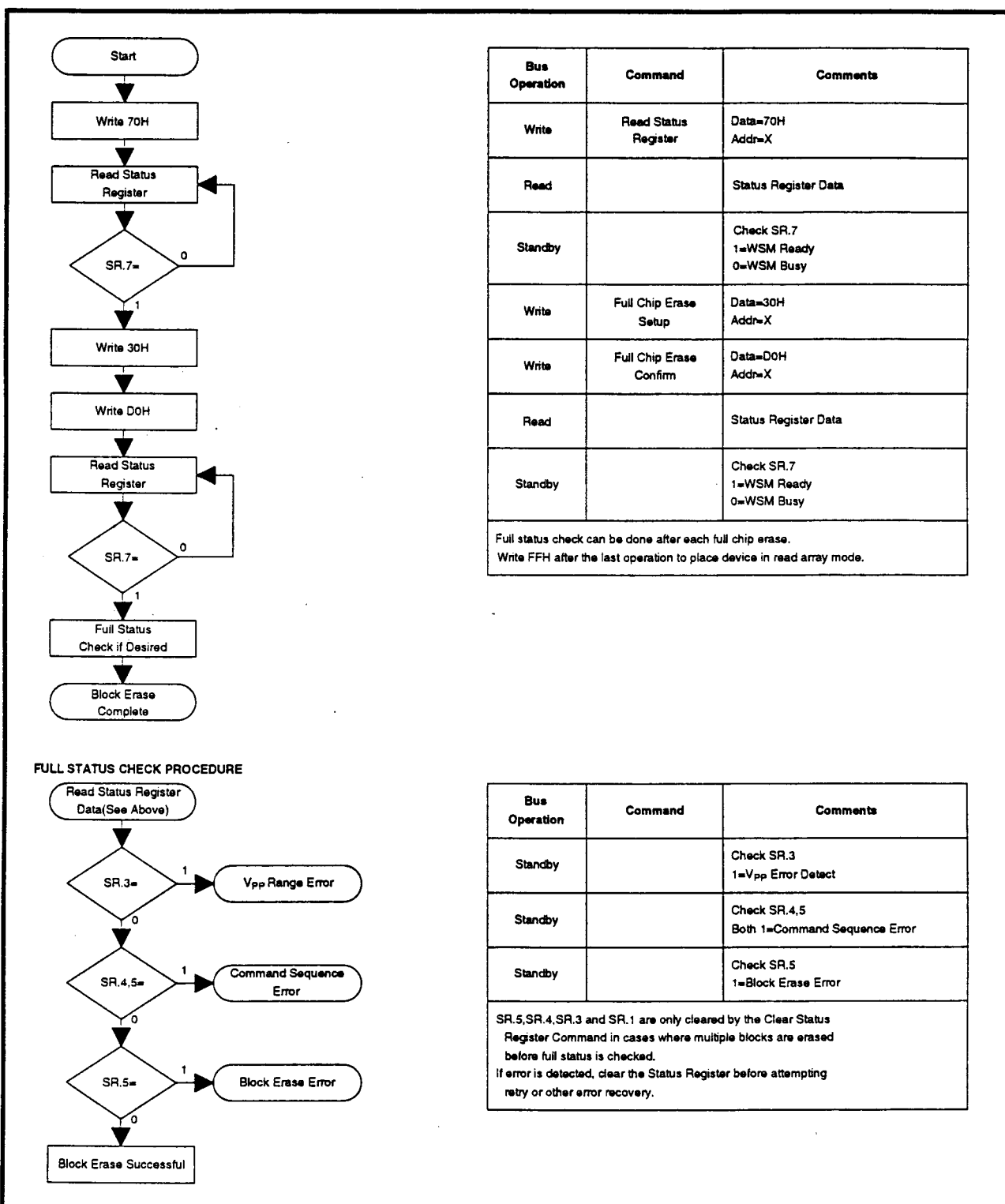
Figure 10. Automated Full Chip Erase Flowchart
