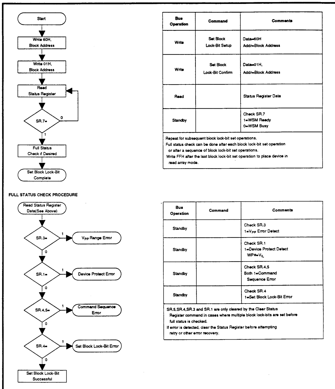
Figure 16. Set Block Lock-Bit Flowchart
