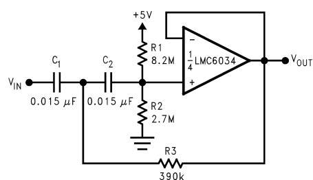
Figure 29. 10 Hz Bandpass Filter
