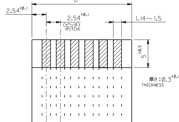
適合F.F.C.推奨寸法 APPLICABLE FFC RECOMMENDED DIMENSION
