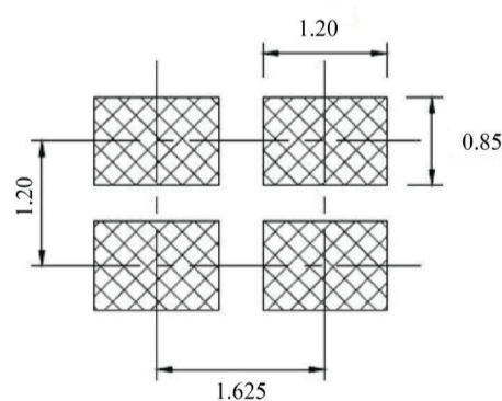
RECOMMENDED LANDING PATTERN DIMENSIONS: mm
