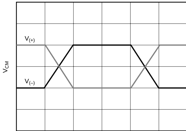
Figure 1. Bus Voltage
