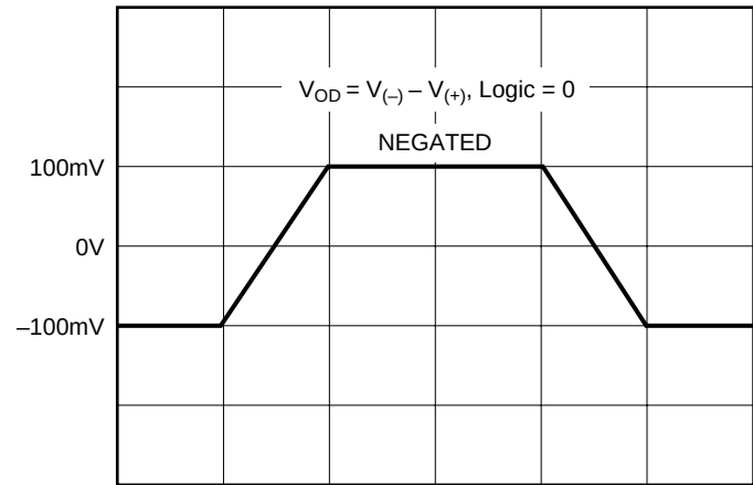
Figure 2. V_{OD}
