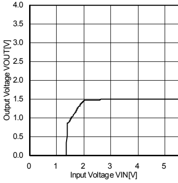
Fig. 1 Output Voltage vs Input Voltage (BH15RB1WGUT)
