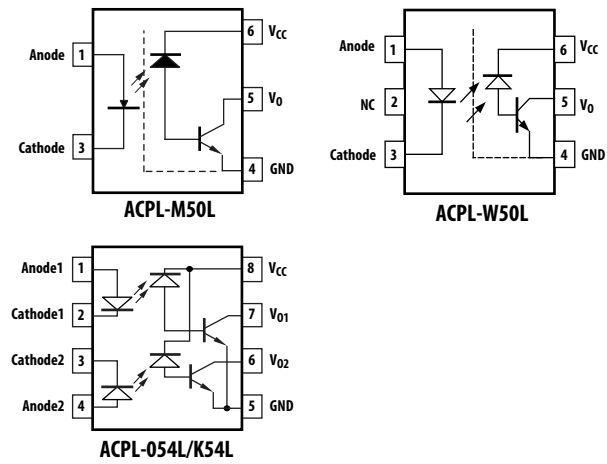
Figure 1 Functional Diagram
