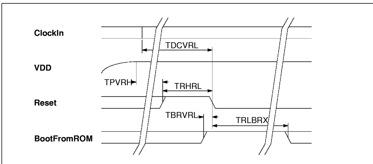
Figure 4.4 Transputer Reset timing with Analyse low
