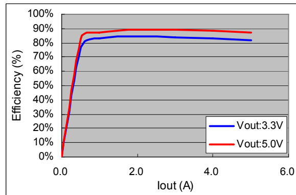
Efficiency (Vin = +12V)
