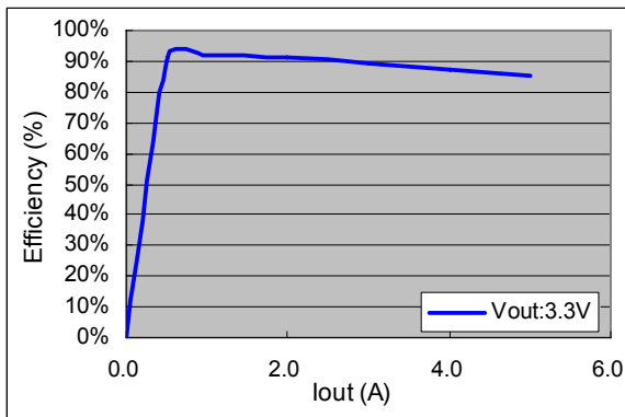
Efficiency (Vin = +5V)
