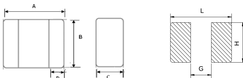
Recommended PCB Pattern
