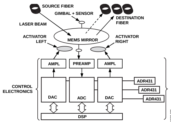
Figure 37. All Optical Router Network
