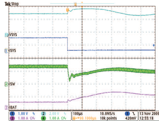
0-A - 1-A Transient on V sys V BUS = 5.5 V V BAT = 3.2 V V OREG = 4 V I CHARGE = 950 mA I IN_limit = 975 mA
