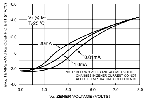
FIG.8- EFFECT OF ZENER CURRENT
