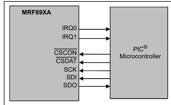
FIGURE 3-32: HOST MCU CONNECTIONS IN PACKET MODE
