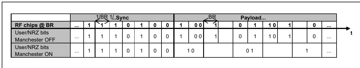
FIGURE 3-30: MANCHESTER ENCODING/DECODING
