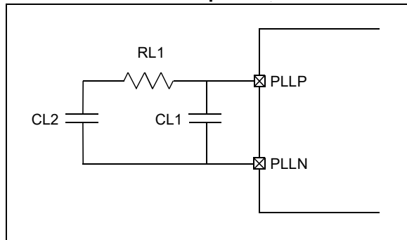
FIGURE 4-7: Loop Filter
