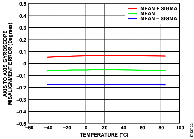
Figure 13. Axis to Axis Gyroscopic Misalignment Error vs. Temperature, All Axes
