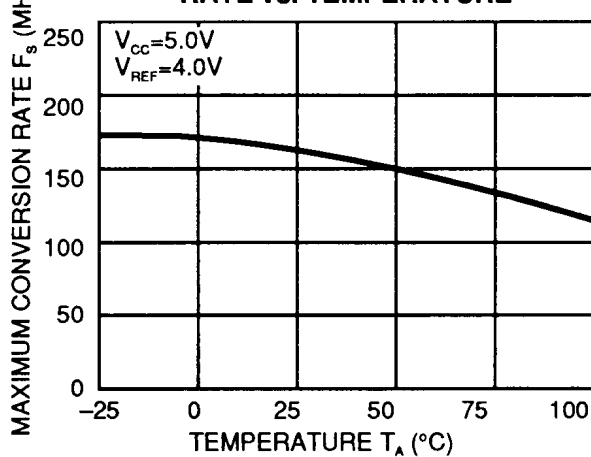
Fig. 16 – MAXIMUM CONVERSION RATE vs. TEMPERATURE
