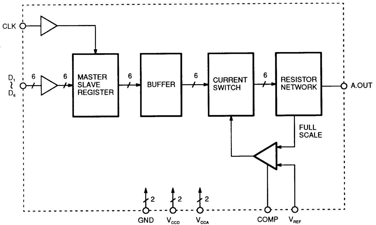
Fig. 1 – BLOCK DIAGRAM
