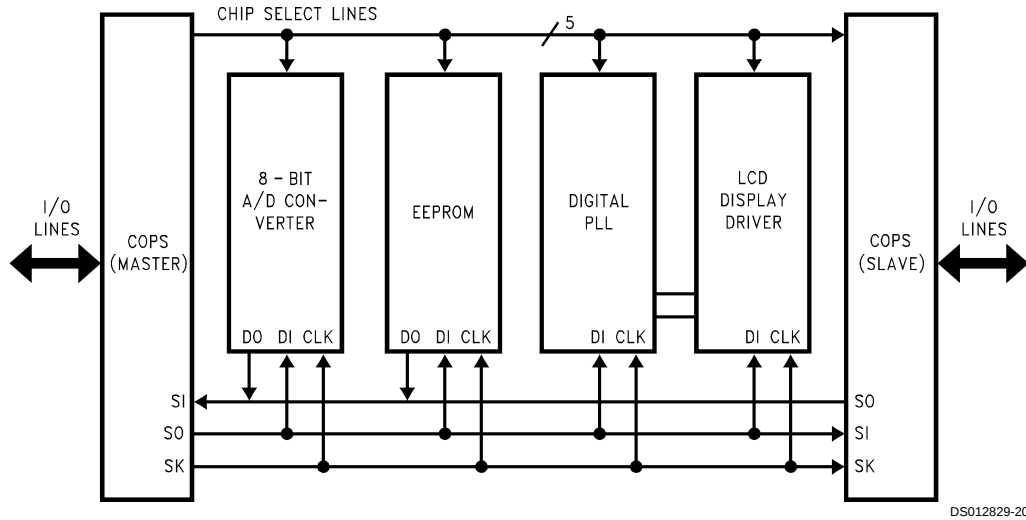
FIGURE 20. MICROWIRE/PLUS Application
