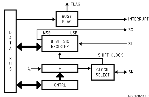
FIGURE 19. MICROWIRE/PLUS Block Diagram
