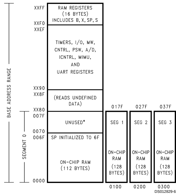
FIGURE 5. RAM Organization
