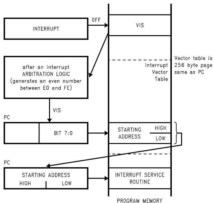
FIGURE 17. VIS Operation
