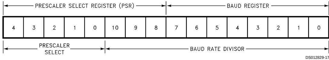
FIGURE 15. USART Baud Clock Divisor Registers
