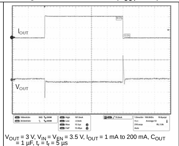
Figure 29. Load transient ( V_{OUT} = 3\text{ V} )
