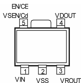
SOT-89-5 (TOP VIEW)
