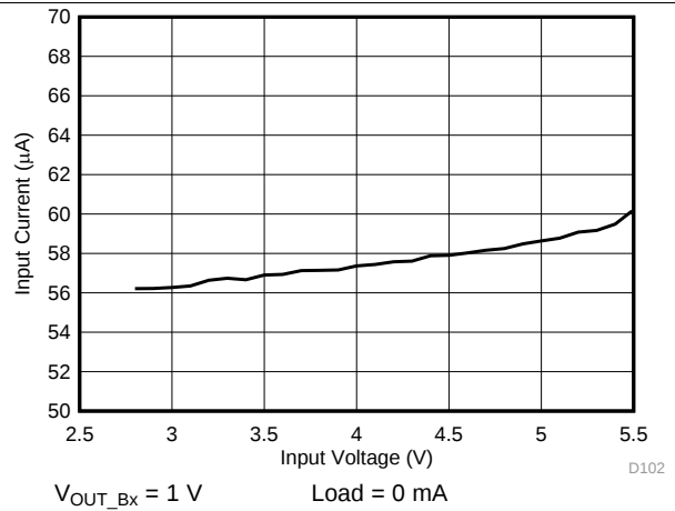
Figure 3. Active State Current Consumption vs Input Voltage, One Buck Regulator Enabled in PFM Mode
