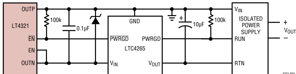
Figure 4. PD Interface Using the \overline{\text{EN}} Pin
