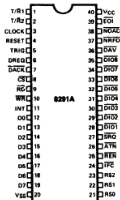
Figure 2. Pin Configuration
