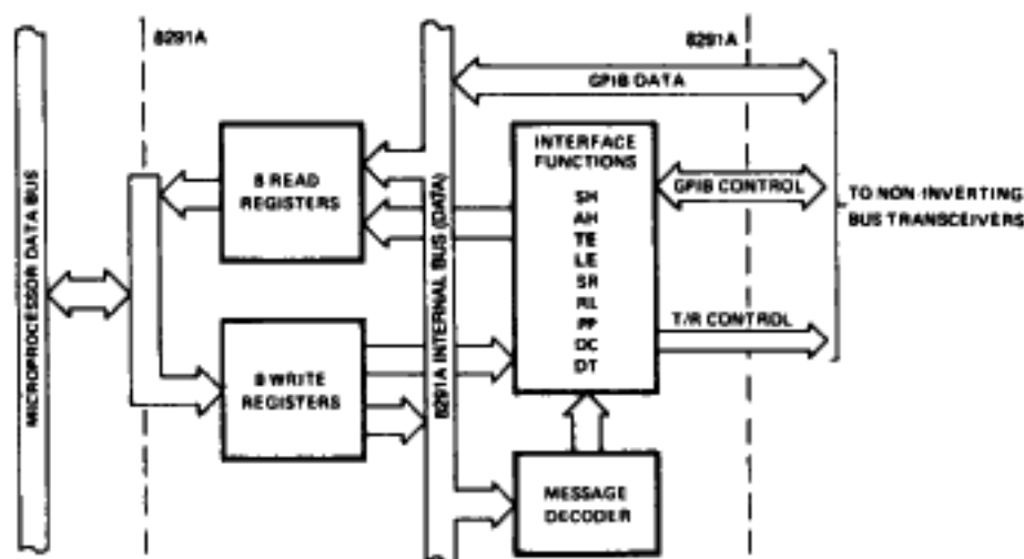
Figure 1. Block Diagram
