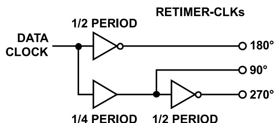
Figure 95. RETIMER-CLK Phases
