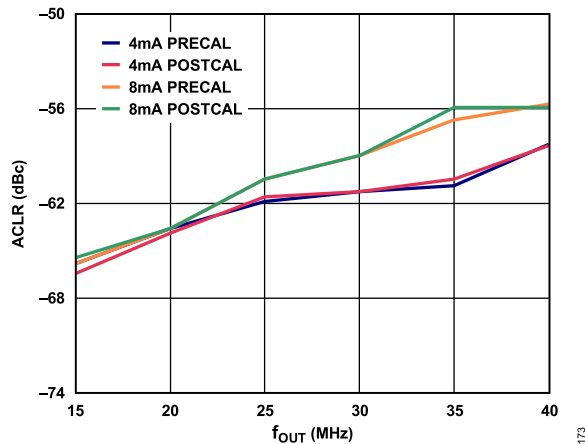
Figure 73. AD9117 Two-Carrier W-CDMA First ACLR vs. f_{OUT} , 1.8 V
