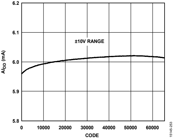
Figure 53. Supply Current ( I_{DD} ) vs. Code
