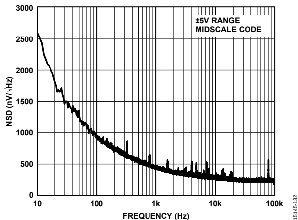
Figure 45. Noise Spectral Density (NSD) vs. Frequency
