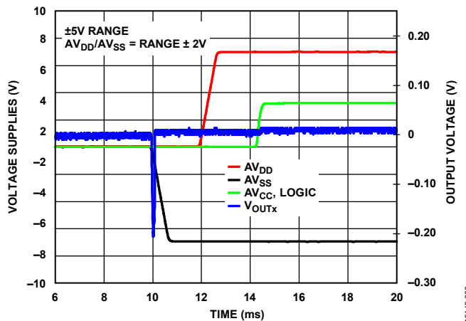
Figure 32. Power-Up Glitch
