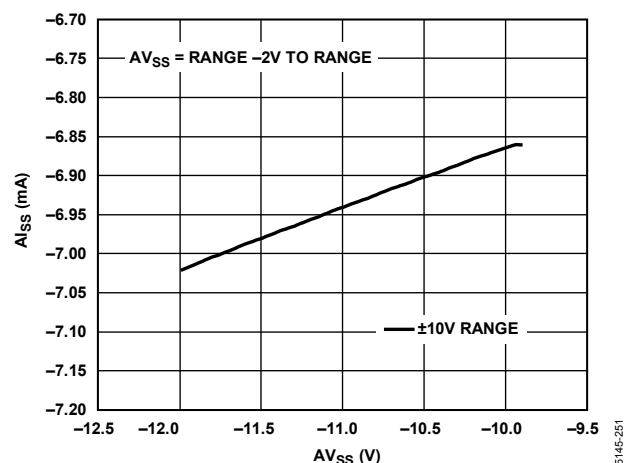
Figure 51. Supply Current ( I_{SS} ) vs. Supply Voltage ( AV_{SS} )
