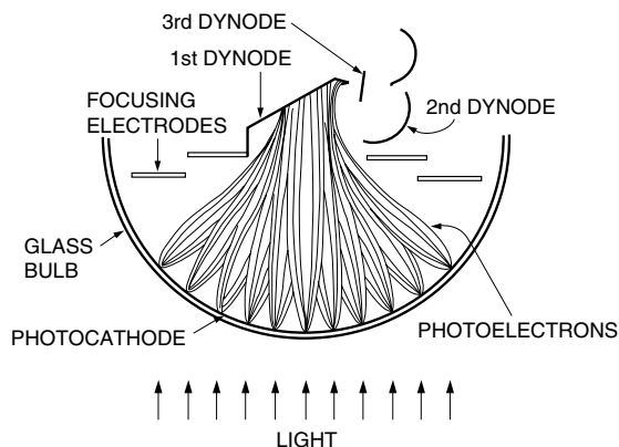
Figure 1: Electron Trajectories
