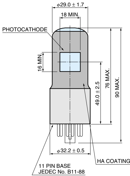
Figure 9: Dimensional Outline and Basing Diagram (Unit: mm)
