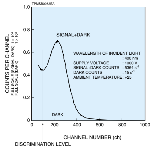
Figure 6: Typical Single Photoelectron Pulse Height Distribution (R2693P)
